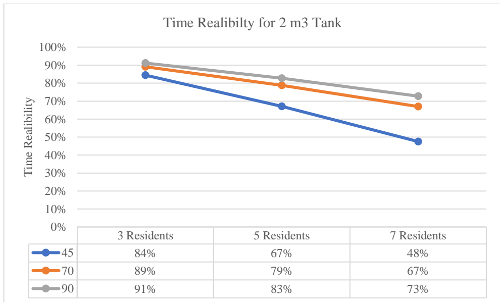
Figure 3. Graph of time reliability comparison for a 2 m³ tank volume.
